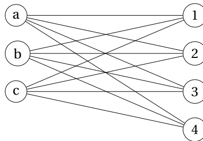
FIGURE 15.7 – Graphe biparti complet K_{3,4}
