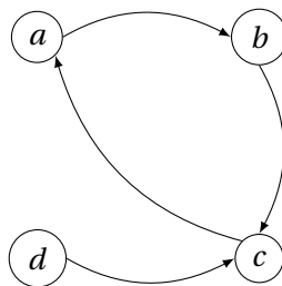
FIGURE 15.4 – Graphe orienté
