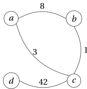
FIGURE 15.3 – Graphe pondéré
