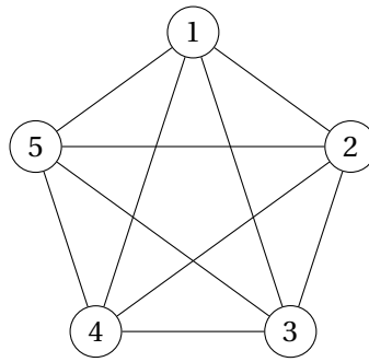
FIGURE 15.5 – Graphe complet K_5
