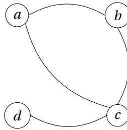
FIGURE 15.1 – Graphe simple
