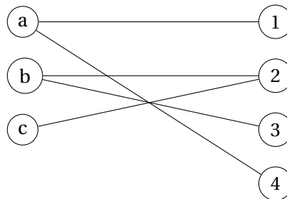
FIGURE 15.6 – Graphe biparti
