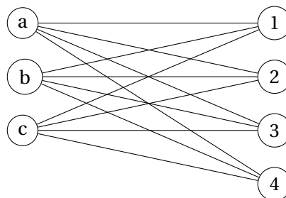
FIGURE 14.7 – Graphe biparti complet K_{3,4}
