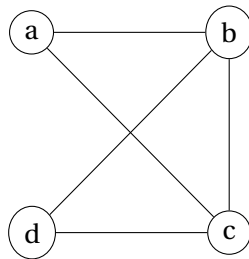
FIGURE 14.12 – Graphe d'exemple G = (S = \{a, b, c, d\}, A = \{ab, ac, bc, bd, dc\})
