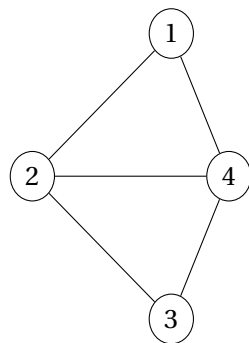
FIGURE 14.13 – Graphe d'exemple G' = (S' = \{1, 2, 3, 4\}, A' = \{12, 14, 24, 23, 43\})
